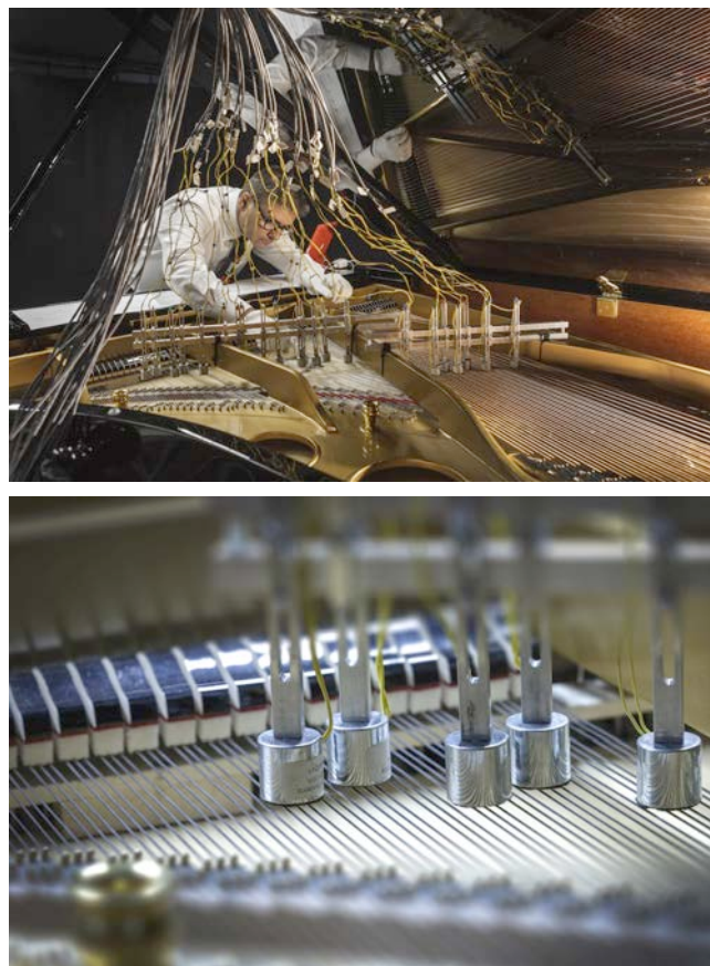
Figure 4: Top: Composer Eduardo R. Miranda preparing the piano for the biocomputer. Bottom: The biocomputer plays the piano through electromagnets placed close to the strings.
