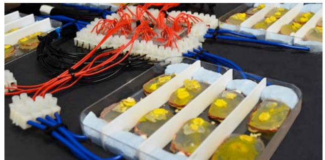
Figure 3: Growing circuit boards for ICCMR's biocomputer.
