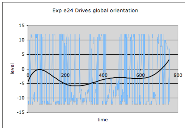
Figure 8: Evolution of the drives-pool global orientation, integration (positive values), expression (negative values) in experiment e24.
