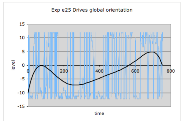
Figure 9: Evolution of the drives-pool global orientation, integration (positive values), expression (negative values) in experiment e25.
